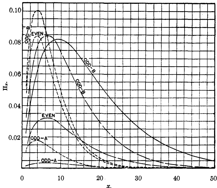
Fig. 6.—Weight fraction distribution curves for a 25% excess of B groups ( r = 0.80 ). When p = 0.85 ----, p = 0.95 - - - and p = 1.00 ———. Curves labeled “even” are for even molecules, i. e. , those having an even number of segments; those labeled “odd-A” are for odd molecules having A groups as termini, and those labeled “odd-B” are for odd , B terminated molecules. The even curves apply for even integers only, the odd curves for odd integers only. One square = 0.005 weight fraction.
